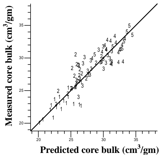
Figure 3. Plot of measured core bulk against predicted core bulk for the samples subjectively assessed for lustre grade with the lustre grade indicated for each sample. 1 = High lustre to 5 = Low lustre.
